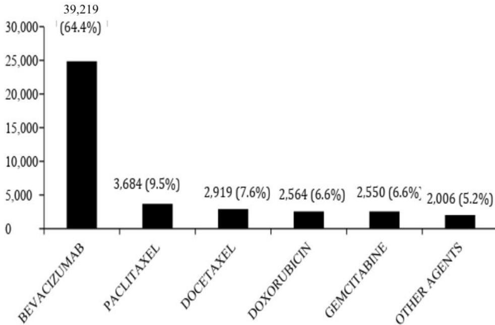
Figure 2: Average cost Anti neoplastic Agents
