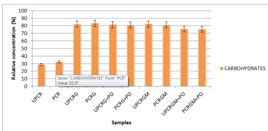
Figure 6: Carbohydrate contents of cassava roots, garri and garri meals
