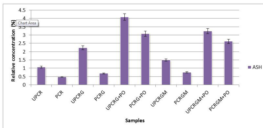
Figure 4: Ash values of cassava roots, garri and garri meals
