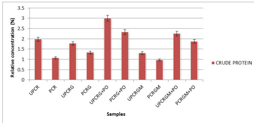
Figure 2: Crude protein contents of cassava roots, garri and garri meals
