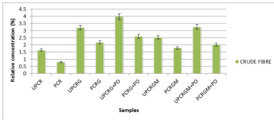
Figure 3: Crude fibre contents of cassava roots, garri and garri meals
