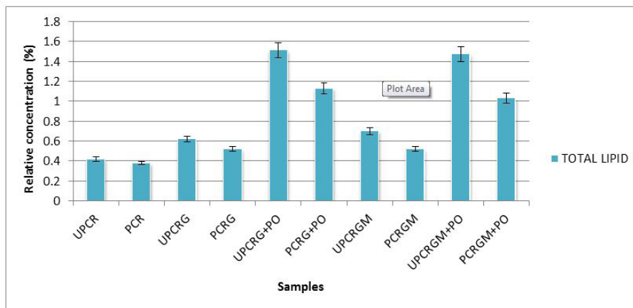
Figure 5: Total lipid contents of cassava roots, garri and garri meals
