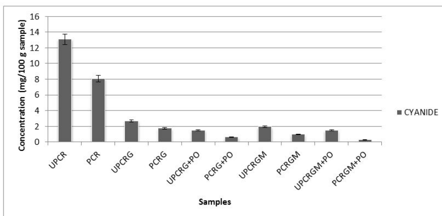
Figure 7: Cyanide contents of cassava roots, garri and garri meals
